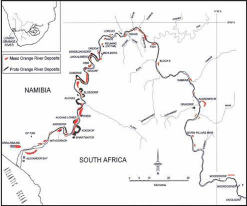
Figure 20: Location of alluvial diamond mines and deposits in terraces of the Proto-Orange
