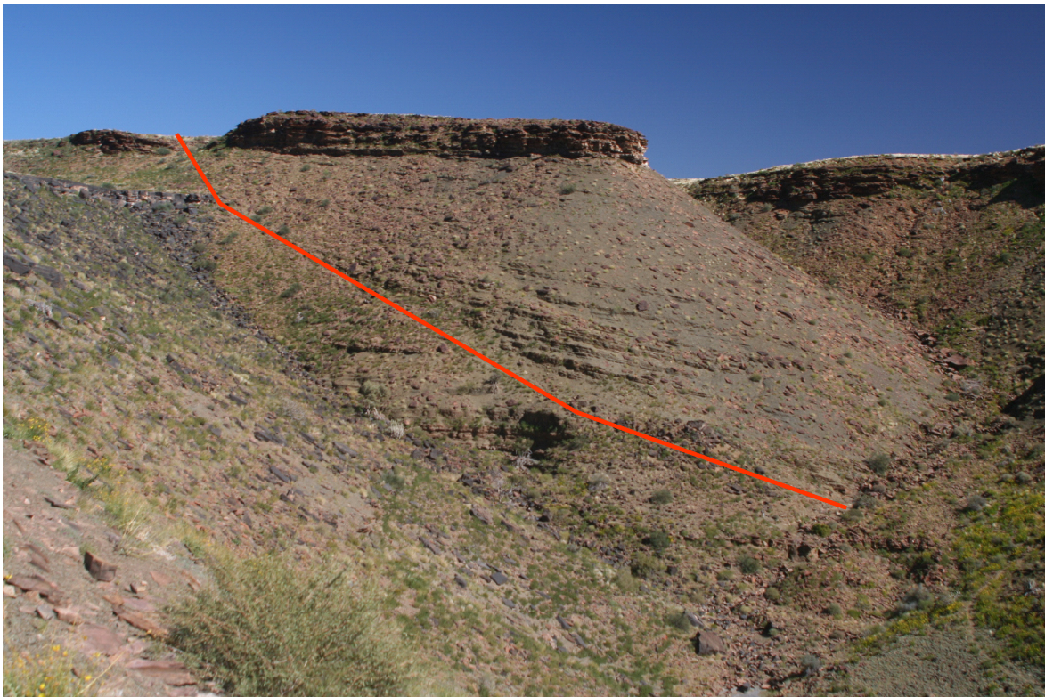
Figure 26: Incised palaeocanyon, marked in red, that immediately post-dates the Precambrian-Cambrian boundary
